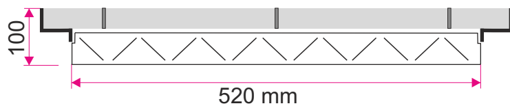
Floor grille and damper with counter running blades KPP-1 + GP
